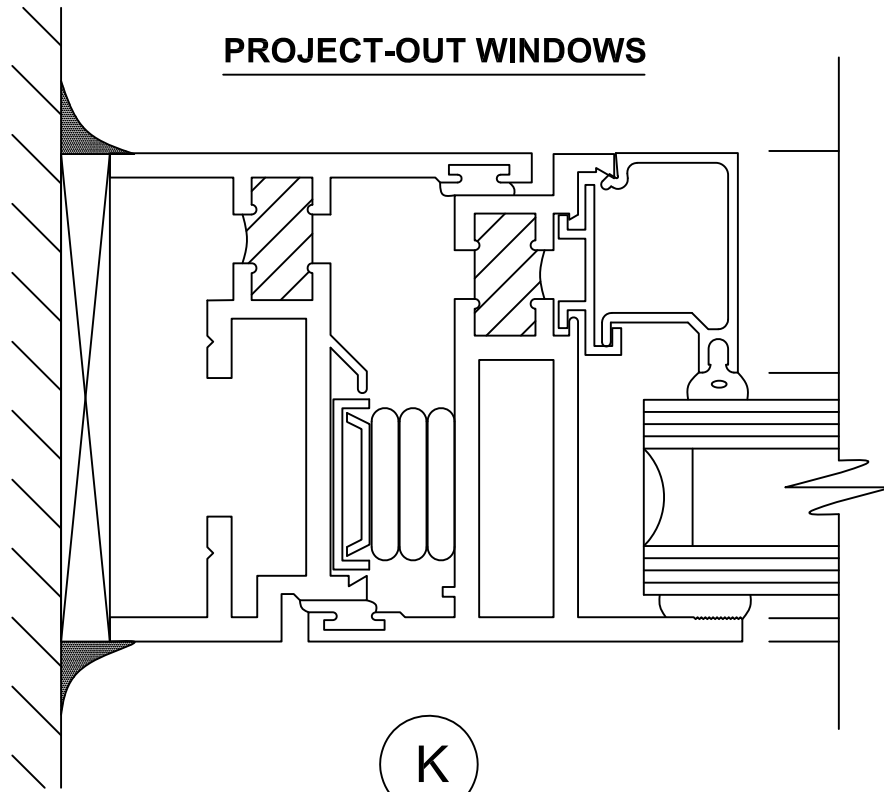
JAMB AT SASH
