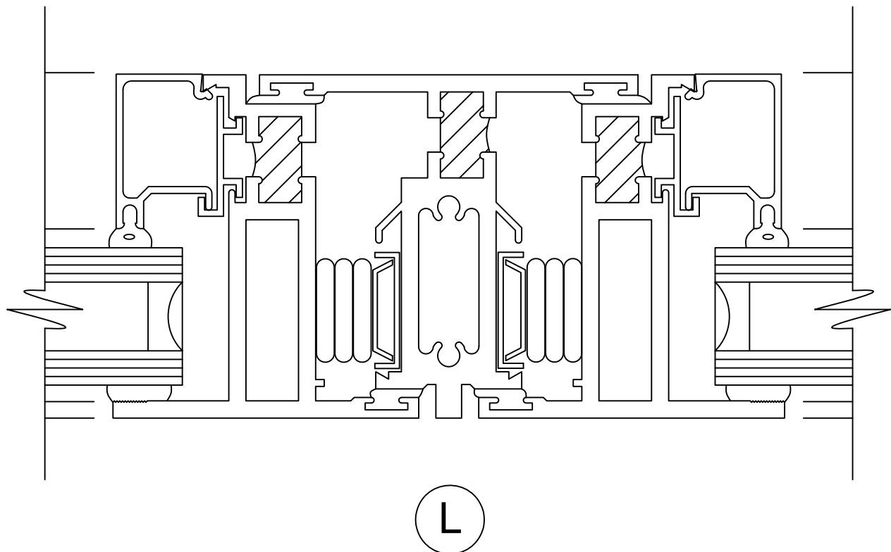
JAMB AT SASH
