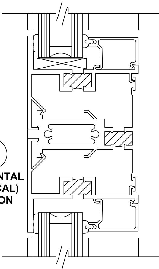
D SILL AT SASH
