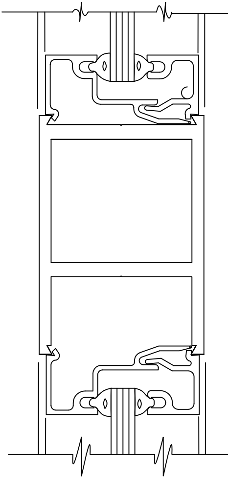
2-1/2" MID RAIL
